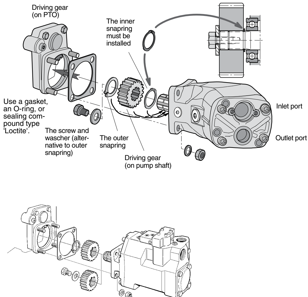
Fig. 6. VP1-to-PTO installation.
