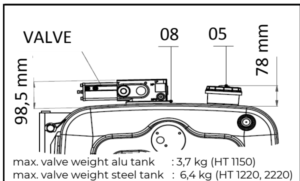
Top mounted valve
