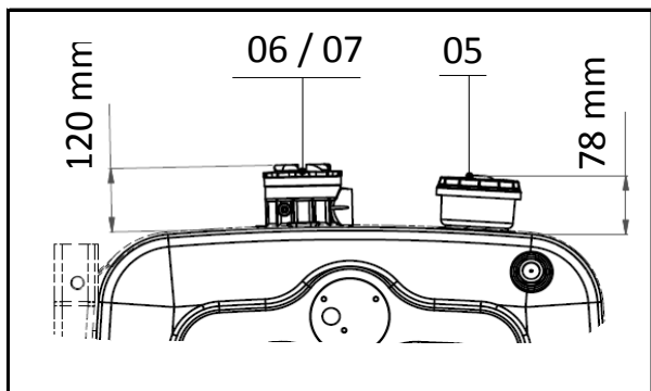
Chassis or cylinder mounted valve
