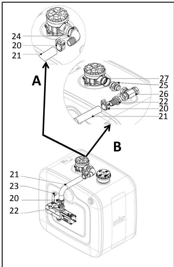
Side mounted valve
